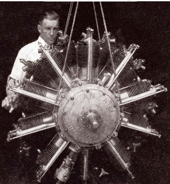
Frank Coffyn with the twentycylinder Anzani motor, imported by Robert Collier in 1913, which would propel a ship at the amazing speed of eighty miles an hour.
