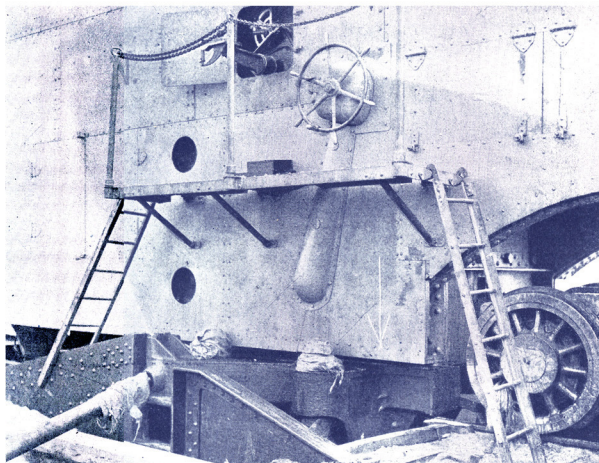
The gun-car resting on the pit foundation. Note the wheel on the side of the car controlling the elevating gear. Upon this foundation, the guns can be trained on targets nearly thirty miles distant when the special shells for land use are fired.
