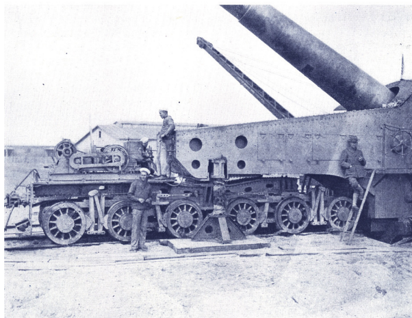
One of the great guns elevated for extreme range. Note the powerful jacks by which the gun car is lifted from its trucks to rest on the pit foundation.
