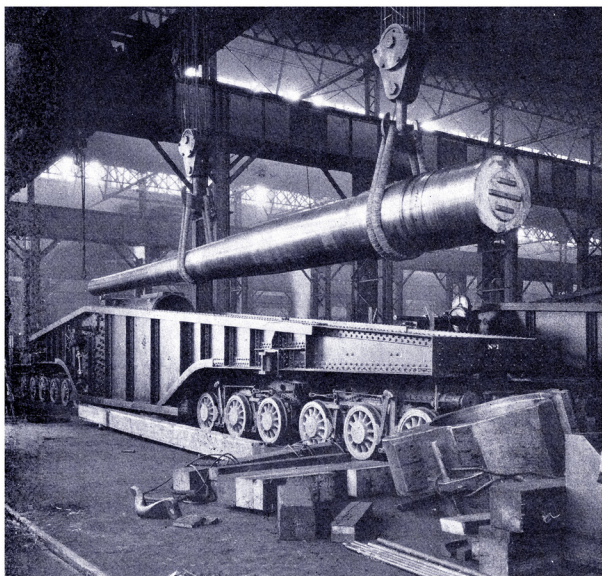
One of the giant weapons being placed by means of a powerful crane in its bed on the colossal girders.
