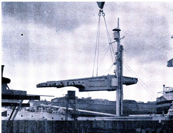
In preparation for the "Battle of St. Nazaire" the great girders were swung ashore from the holds of the ships which carried them to France.
